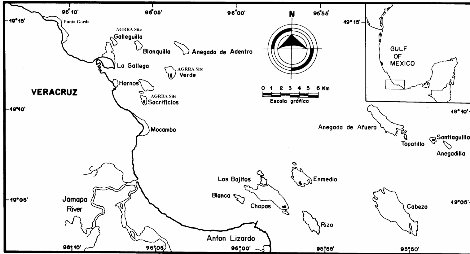
Figure 1. AGRR survey sites in the Veracruz Reef System.
