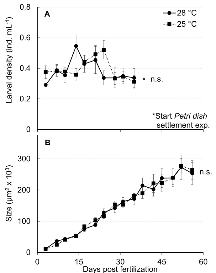
Fig. 6. Experiment 4 (Temperature): The growth and survival of D. antillarum larvae from 3 to 56 DPF fed incrementally depending on DPF with 15,000, 30,000 and 60,000 cells of R. salina \text{mL}^{-1} reared at 28 °C (line) and 25 °C (dotted line), measured data 28.2 \pm 0.1 °C and 24.9 \pm 0.2 °C (average \pm SD, n = 36 ), showing (A) larval density described as number of individuals \text{mL}^{-1} (starting at day 35 larvae were used for petri dish settlement tests, artificially lowering larval density and therefore no longer shown) where both DPF ( F = 2.25 , df = 463 , P = 0.135 ) and temperature ( F = 4.06 , df = 14 , P = 0.064 ) were no significant predictors and (B) body size ( \mu\text{m}^2 \times 10^3 ) where DPF ( F = 4026.94 , df = 1267.47 , P \leq 0.001 ) was a significant predictor but temperature was not ( F = 24.86 , df = 1.13 , P = 0.297 ). N.s. indicates there was no significant difference ( n = 8 ).
