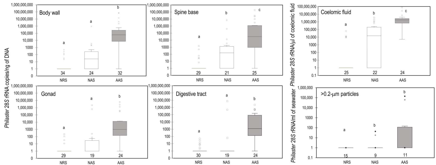
Fig. 3. Box plots of Philaster -like 28S rRNA loads determined by qPCR for different sample types (body wall, spine base, coelomic fluid, gonad, digestive tract, and >0.2-μm particles collected immediately above urchins) acquired from different specimen types. The number of specimens surveyed is indicated below box plots. a, b, and c denote groups that are not statistically different (Kruskal-Wallis test with Dunn's post hoc correction for multiple comparisons). The AAS box plots are shaded gray to highlight results from abnormal specimens. NRS, grossly normal at reference site; NAS, grossly normal at affected site; AAS, abnormal at affected site.
